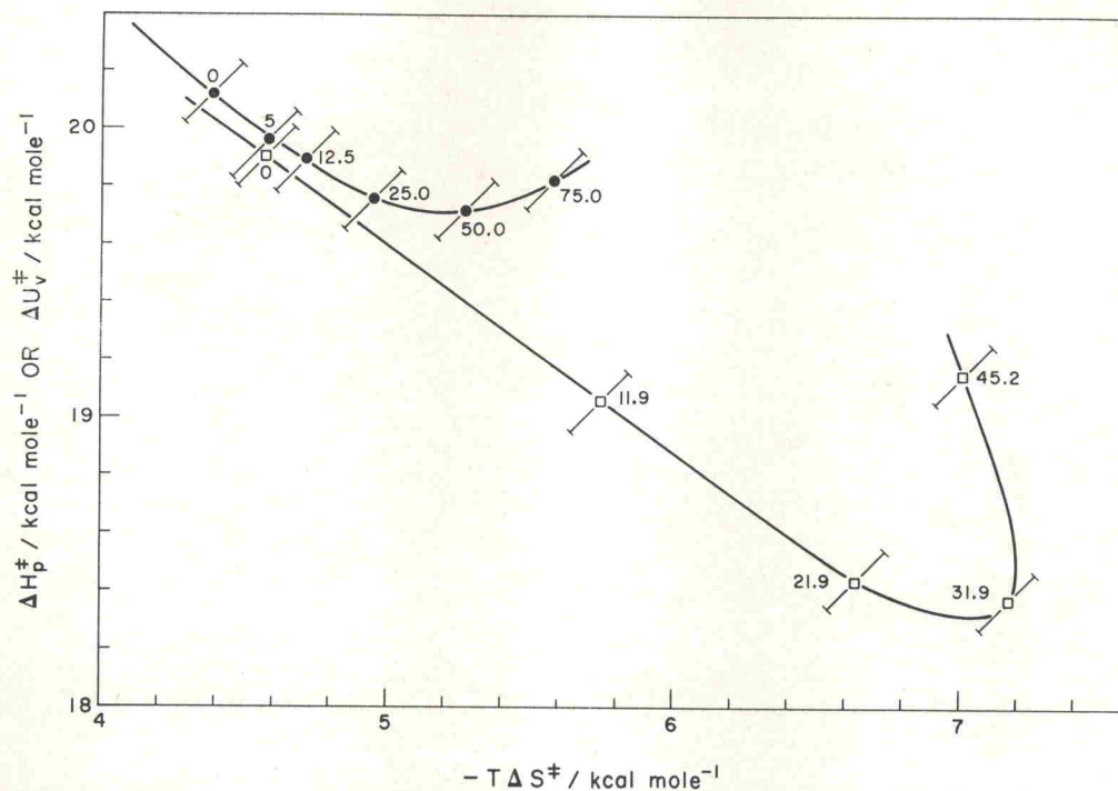
Figure 3. Enthalpy-entropy compensation for the solvolysis of benzyl chloride in water-glycerol and water-ethanol: 10 ●, water-glycerol; □, water-ethanol.
